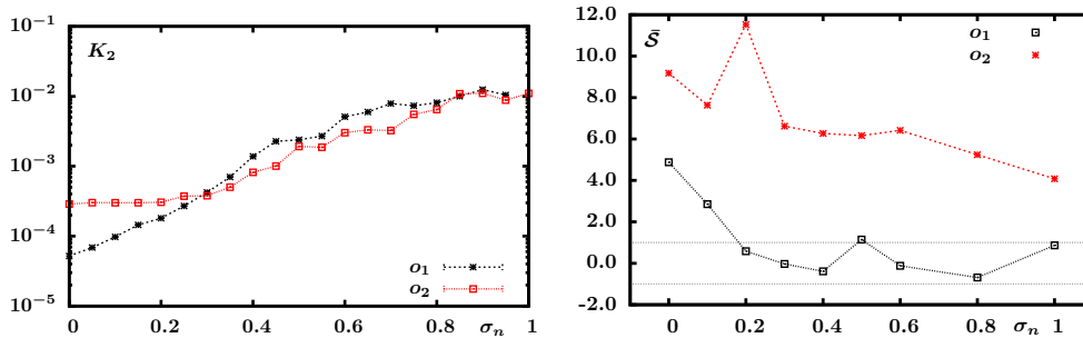
Figure 3. The estimates of the Rényi's entropy K_2 computed for RR~15% and the significance of its comparison with surrogates with increasing strength of the noise.
